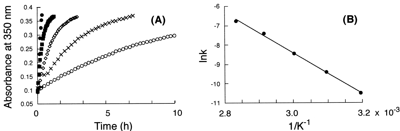
Figure 4. (A) Time-dependent changes in absorbance at 350 nm for photoisomerized oligomer 5 at different temperatures: (○) 80°C, (■) 70°C, (◇) 60°C, (x) 50°C, (○) 40°C. (B) Arrhenius plot for the cis-trans isomerization of oligomer 5 .
