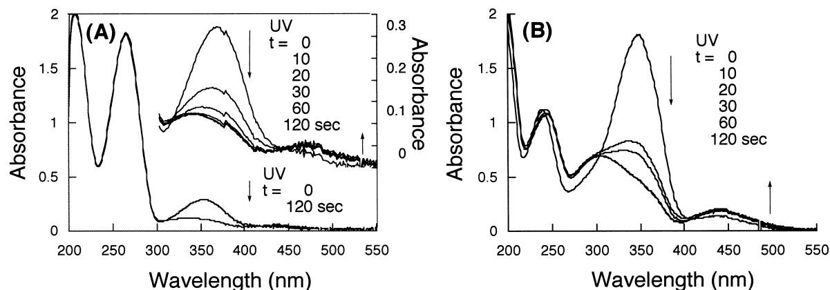
Figure 1. Changes in the UV-vis spectra for azobenzene containing oligonucleotide 5 (A) in a phosphate buffer and its model compound 3a in CH 3 CN (B) due to photoisomerization. The solution of the azobenzene derivative in a Pyrex test tube was irradiated in a cooled water bath (5°C) by a high-pressure Hg lamp using band-path filter to transmit light at around 350 nm. UV-vis spectra were obtained at the same temperature at the indicated time. After 120 s, no further spectral changes were observed for both derivatives.
