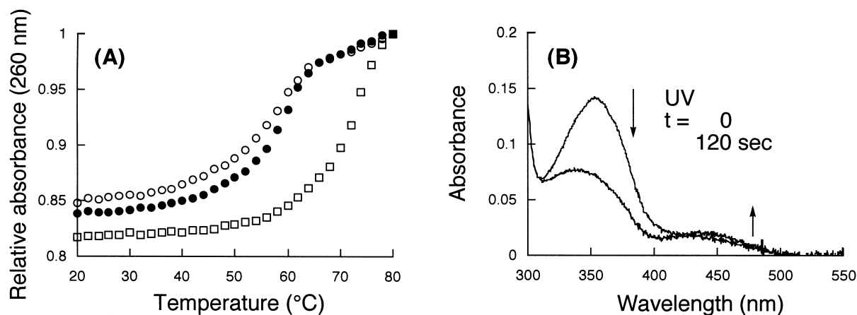
Figure 3. (A) UV melting profiles for duplexes of (●) oligomer 8 , (○) 5'-dCCCTAGGAAAAATCGGATCTCGG (24-mer), and (□) 5'-dCCTAGGTCGGATCTCGG (18-mer) formed with 18-mer target (5'-dCCGAGATCCGACCTAGGG) at a strand concentration of 5 \times 10^{-5} M in 1.0 M NaCl and 0.01 M sodium phosphate, adjusted to pH 7. The melting experiments were carried out without photo-illumination. (B) Changes in the UV-vis spectra for azobenzene containing duplex 8 in the phosphate buffer due to photoisomerization. The photoirradiation was done in the same way as described in Figure 1. After 120 sec, no further spectral changes were observed.
