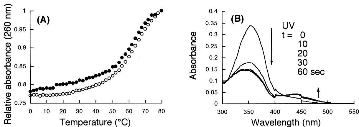
Figure 2. (A) UV melting curves for azobenzene containing oligonucleotide 7 at different strand concentrations (○: 5 \times 10^{-5} M, ●: 1 \times 10^{-5} M) in 0.1 M NaCl and 0.01 M sodium phosphate, adjusted to pH 7. The melting experiments were carried out without photo-illumination. (B) Changes in the UV-vis spectra for azobenzene containing oligonucleotide 7 in the phosphate buffer due to photoisomerization. The photoirradiation was done in the same way as described in Figure 1. After 60 s, no further spectral changes were observed.
